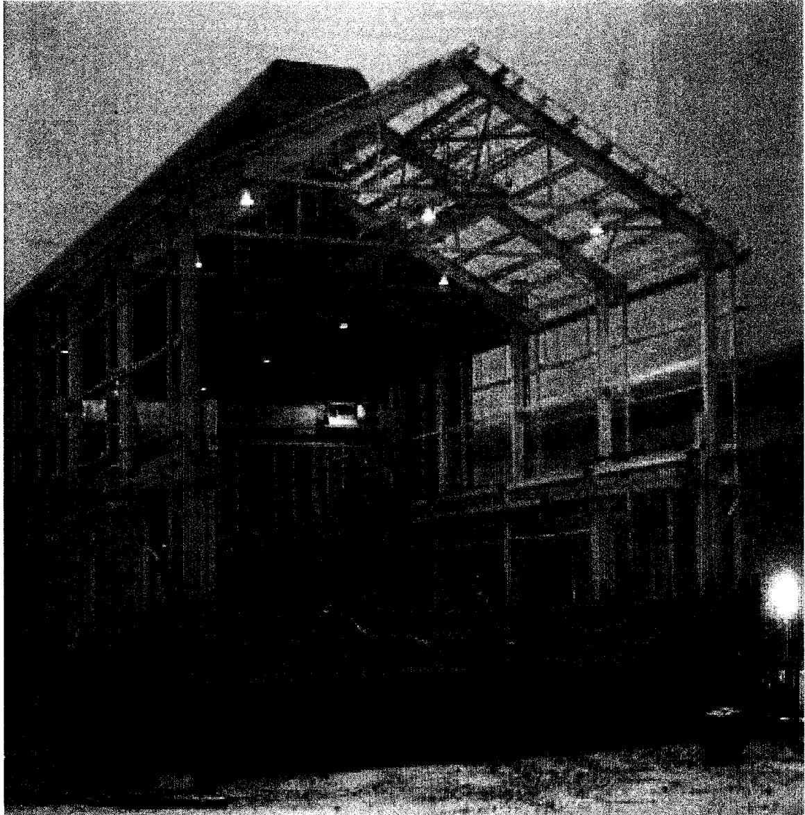
Air-Therm ventilator on potline building
