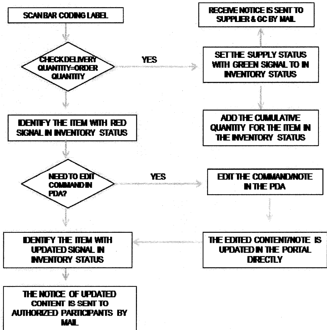
Figure 1.4 Diagram 4 of Mobile Barcode System (from Tseng and Dzeng, 2005)
